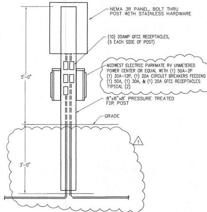
RV POST PANEL TYPE 1 DETAIL
